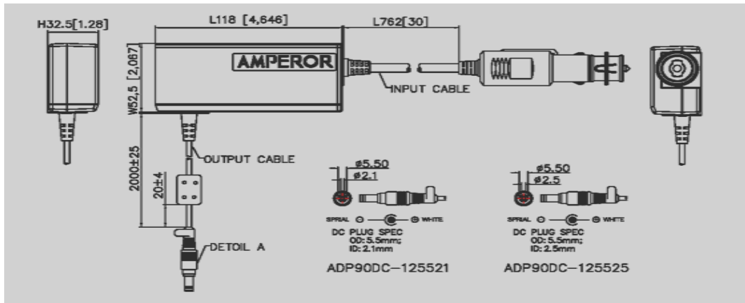
Figure 1: For ADP90DC-125521 and ADP90DC-125525 Model
