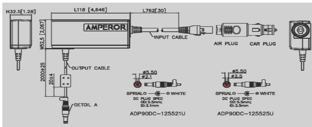
Figure 2: For ADP90DC-125521U and ADP90DC-125525U Model
